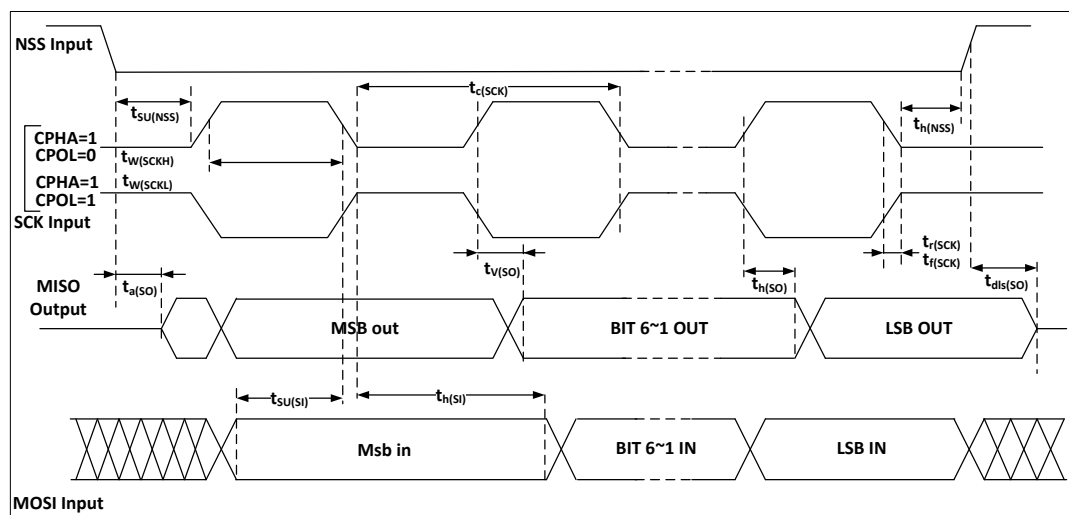
Figure 11 SPI timing diagram—slave mode and CPHA=1(1)
