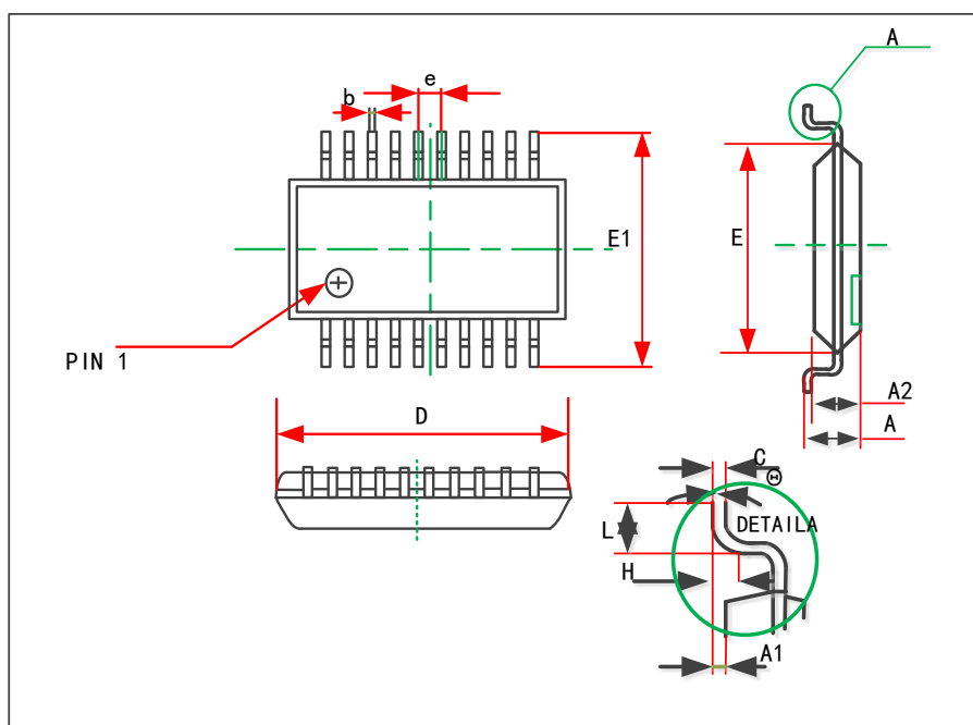
Figure 15 Package diagram of TSSOP20
