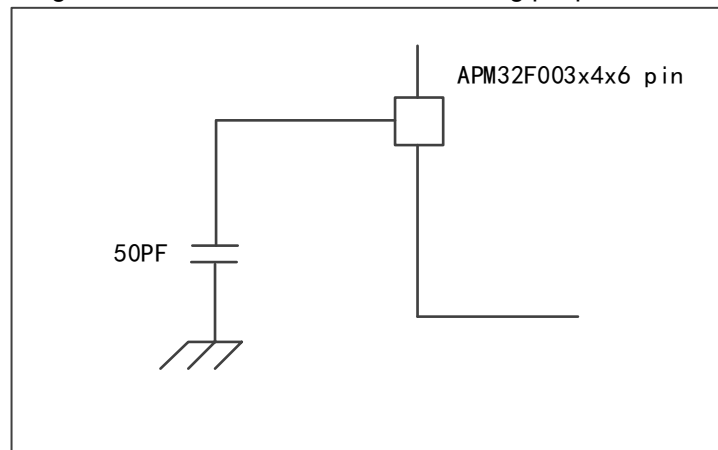
Figure 7 Load conditions when measuring pin parameters
