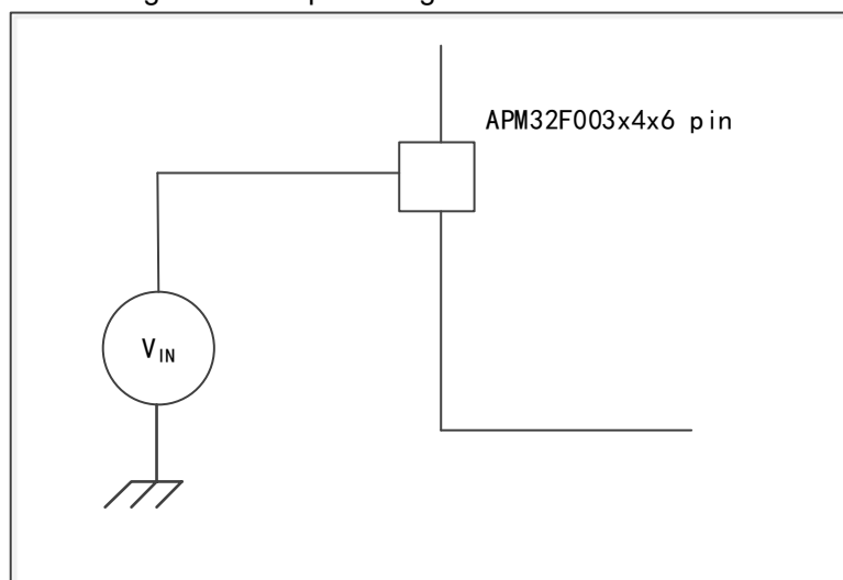
Figure 8 Pin input voltage measurement scheme
