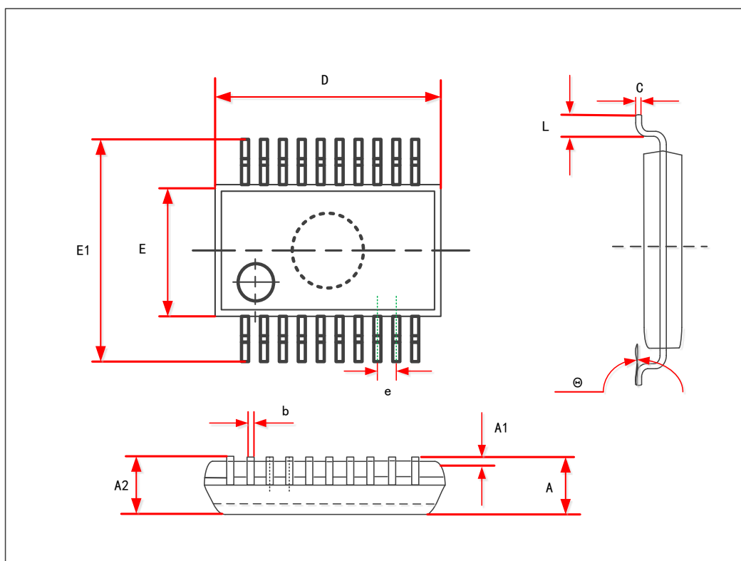
Figure 17 Package diagram of SOP20
