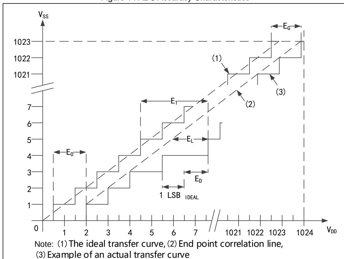
Figure 14 ADC Accuracy Characteristics
