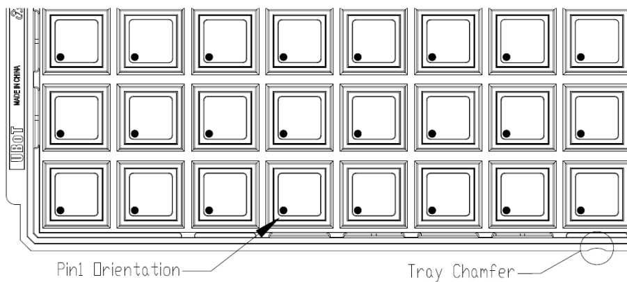
Figure 22 Pin1 Orientation and tray chamfer
