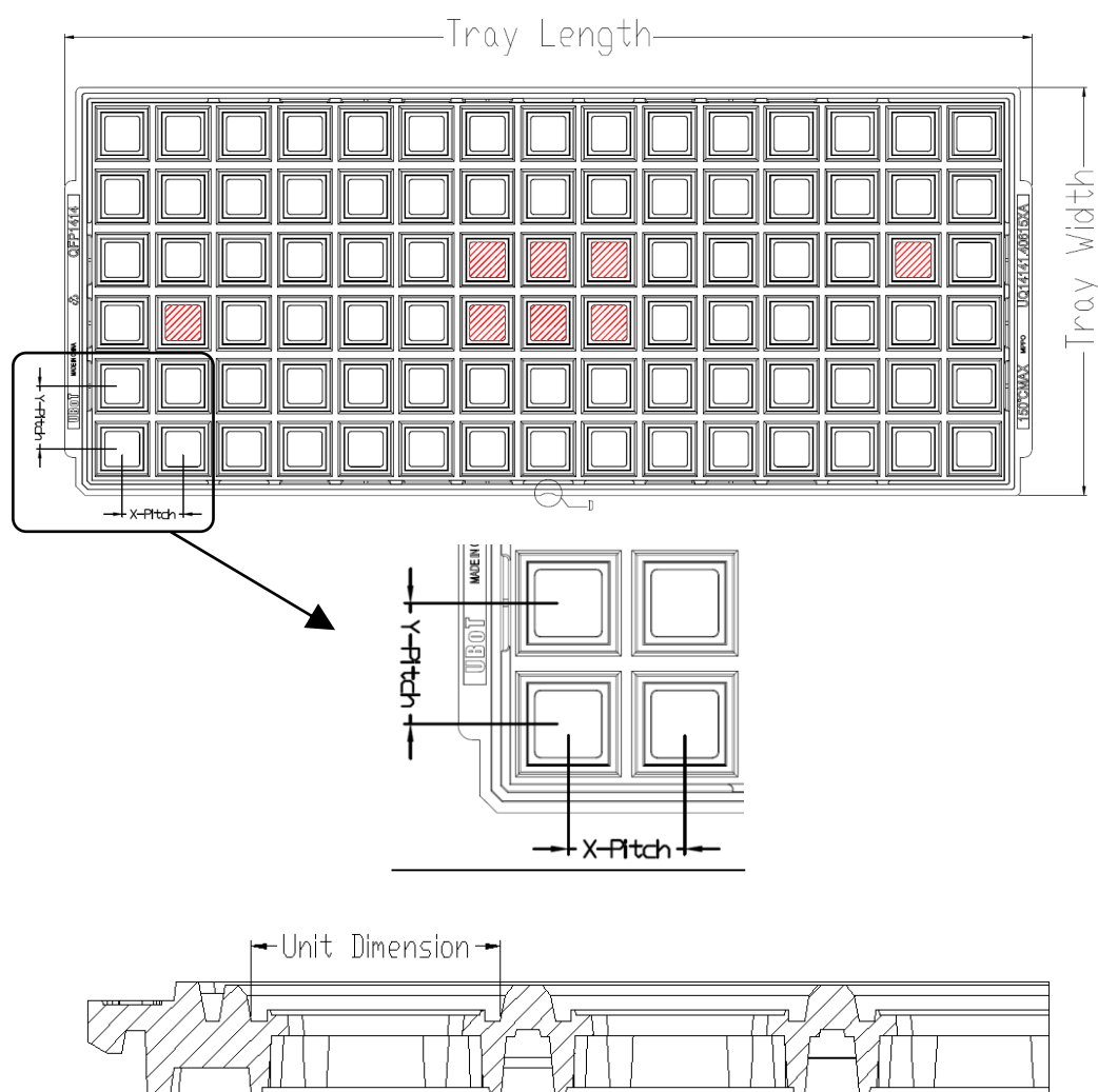
Figure 23 Tray Dimensions
