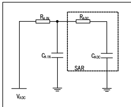
Figure 13 Typical application of ADC
