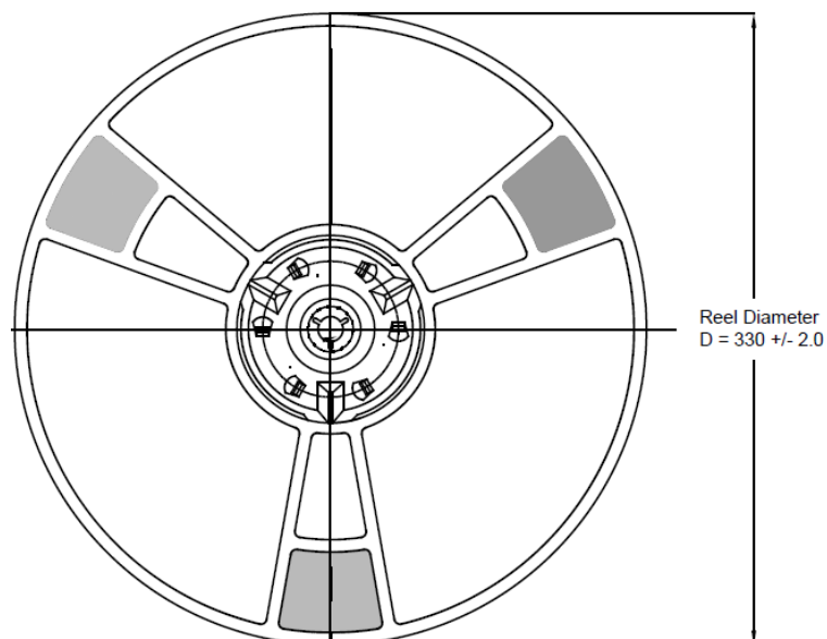
Figure 21 Reel Dimensions
