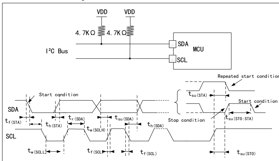
Figure 9 Bus AC waveform and test circuit
