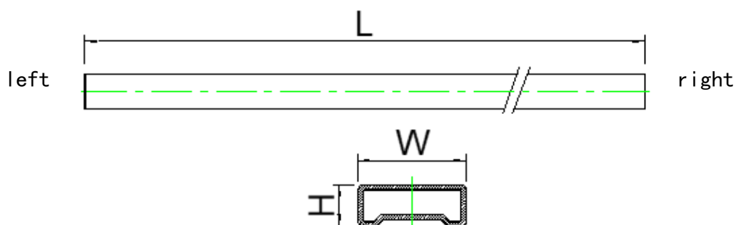
Figure 24 Package drawing of SOP&TSSOP material pipe
