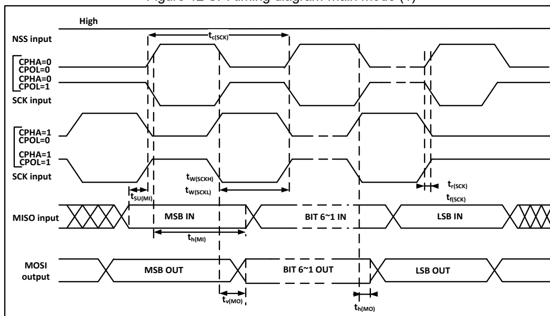
Figure 12 SPI timing diagram-main mode (1)
