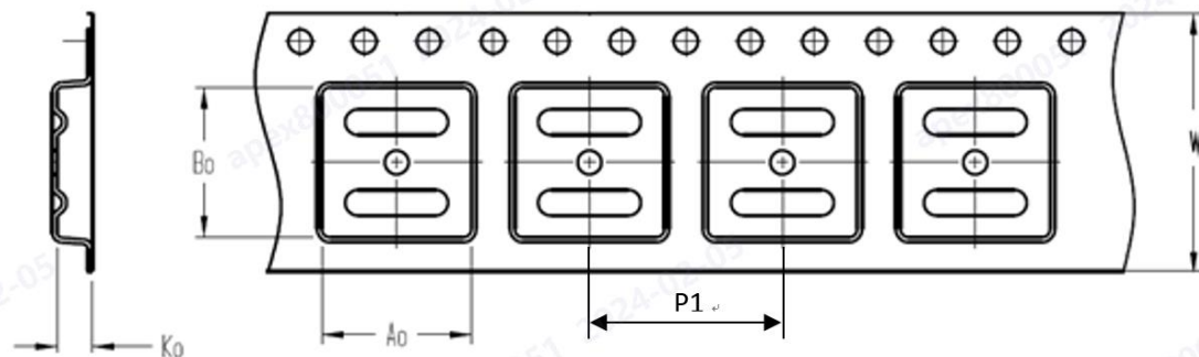
Figure 19 Tape Dimensions
