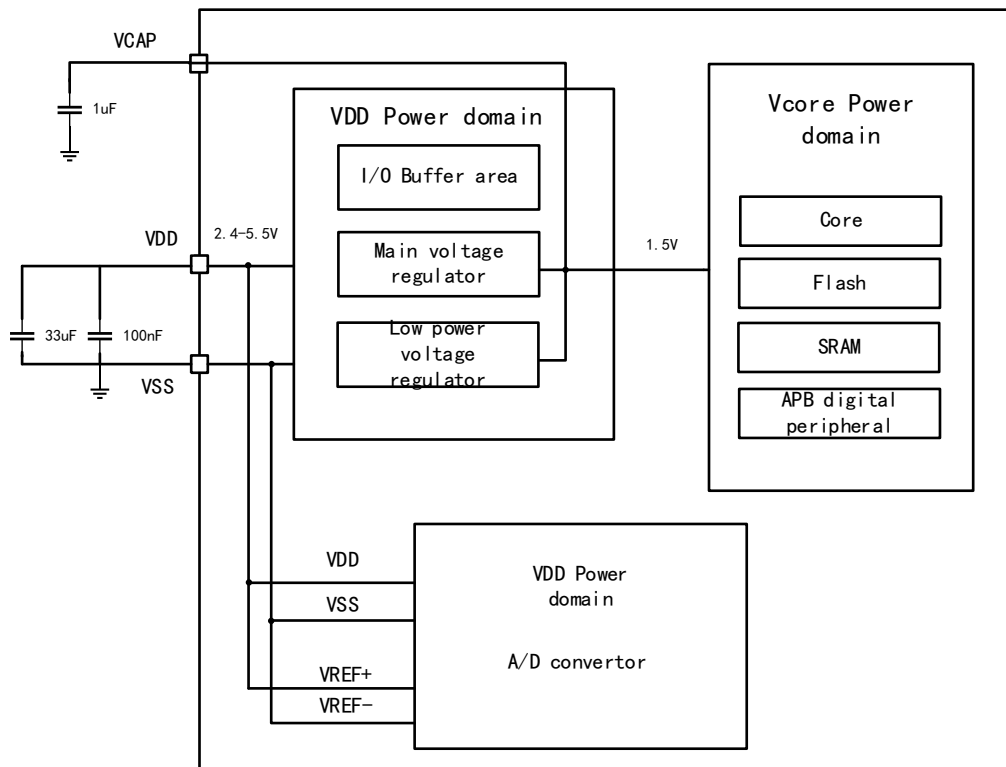
Figure 6 Power Supply Scheme
